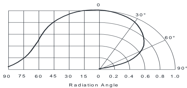
Typical Radiation Pattern 120°
