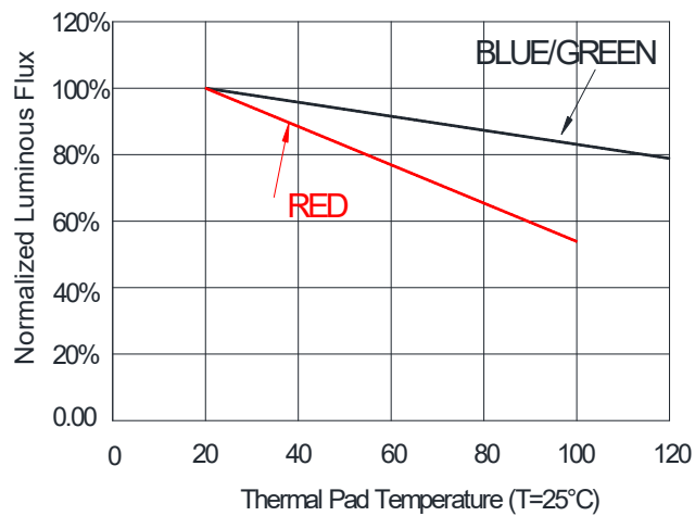
Thermal Pad Temperature vs. Relative Light Output
