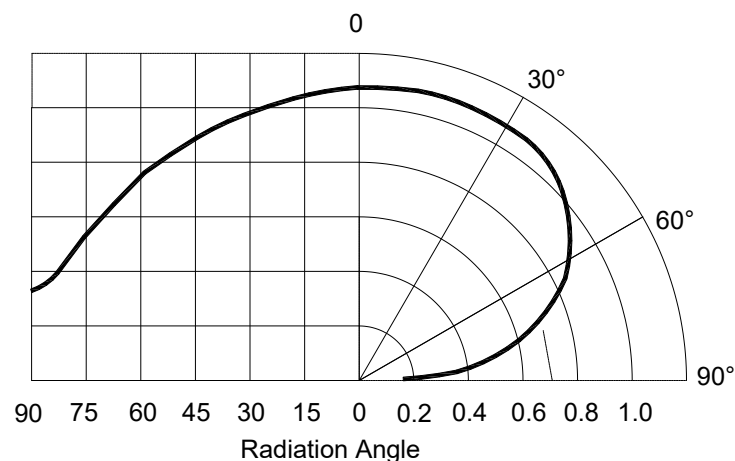
Typical Radiation Pattern 160°
