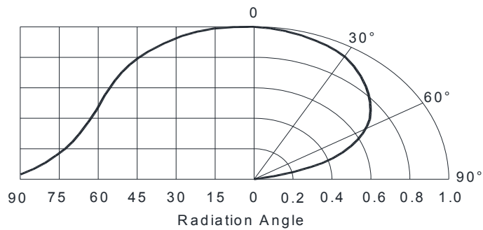
Typical Radiation Pattern 120°
