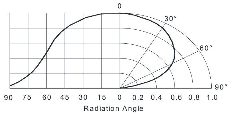
Typical Radiation Pattern 120°
