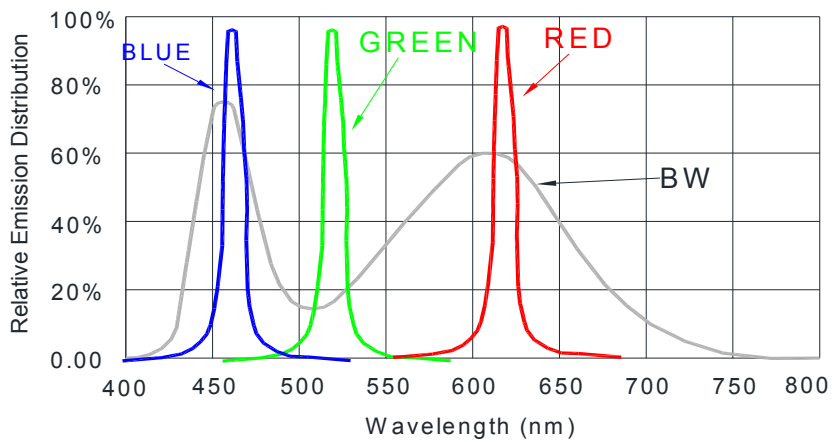
Wavelength Characteristics
