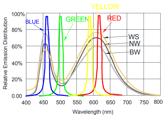
Wavelength Characteristics
